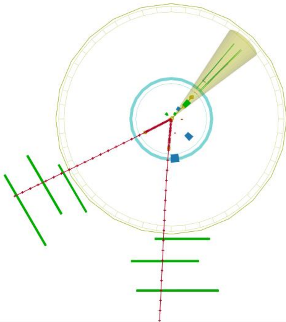
CMS Data Express Event Display
