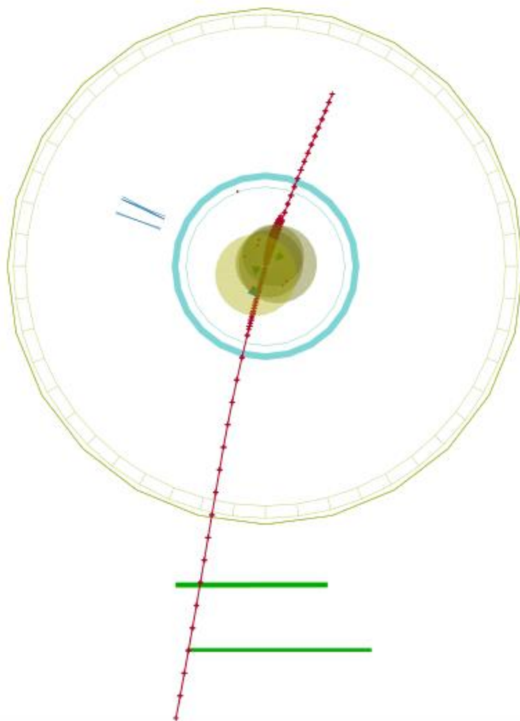
CMS Data Express Event Display
