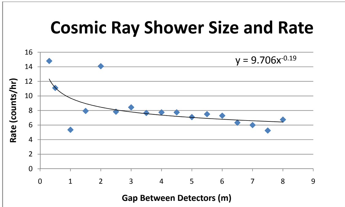
Figure 8. Graph showing relationships between cosmic ray shower sizes and rates. The points represent the rate for each gap between the detectors. A power trendline was fit to the graph, and its equation is 9.706x^{-0.19} .
